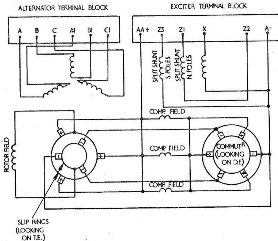
Fig. 3. Internal wiring diagram
