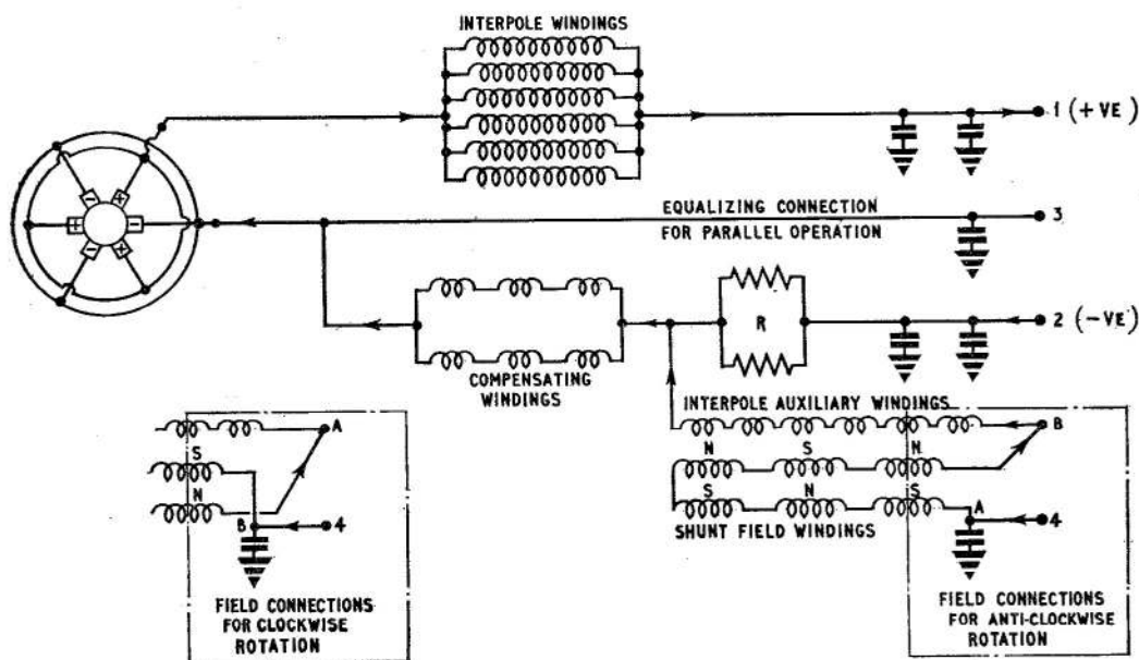
Fig. 4. Circuit diagram
