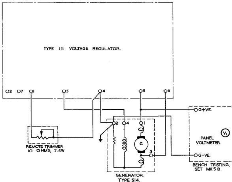
Fig.5 Test circuit
