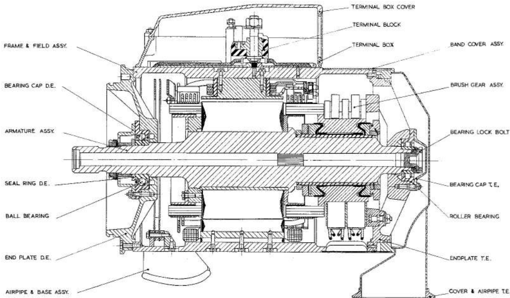
Fig.2 Sectional view
