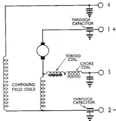
Fig. 2. Terminal arrangement and circuit diagram
