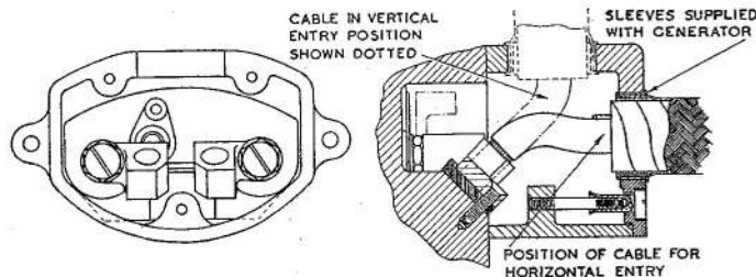
Fig. 3. Terminal box
