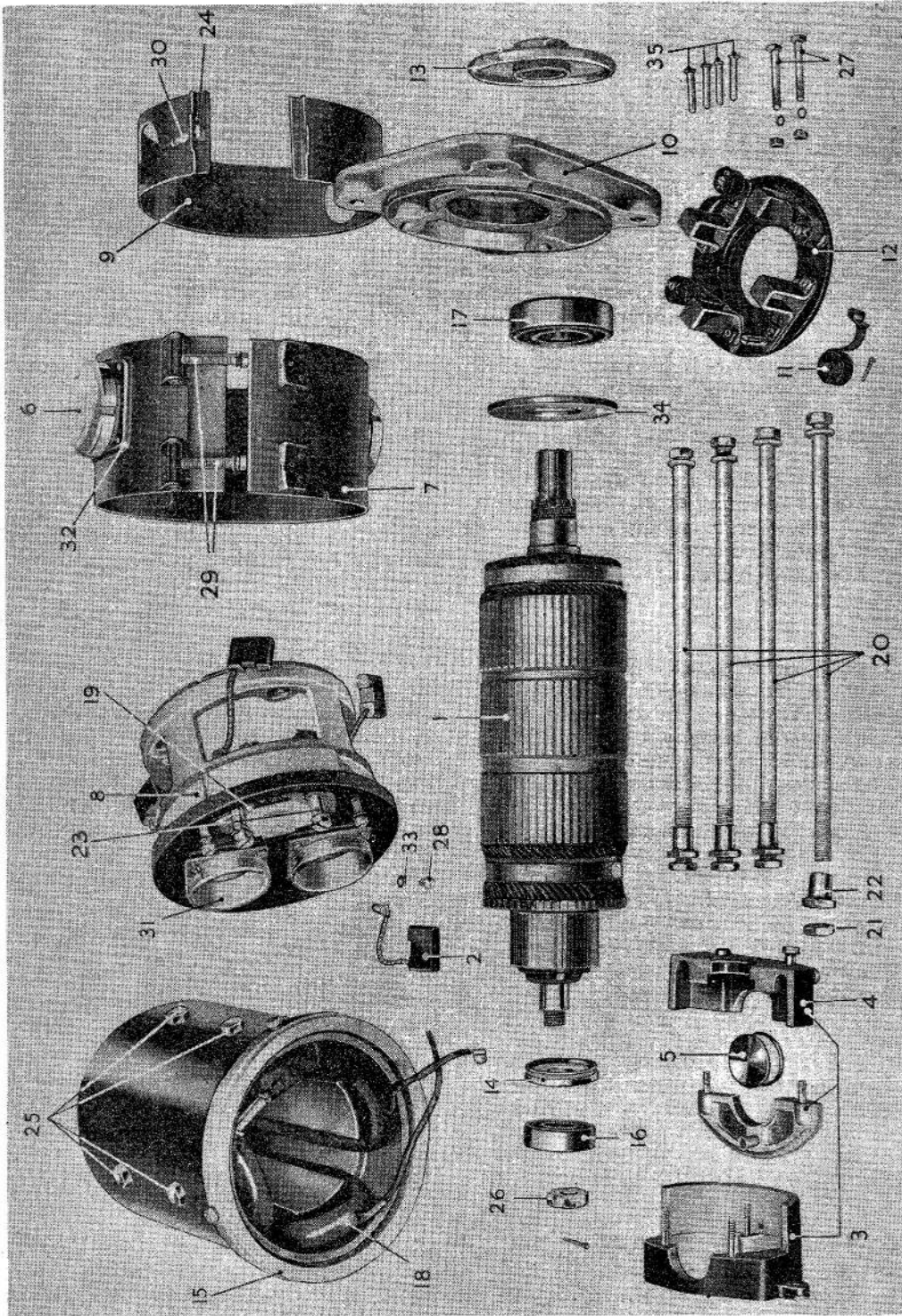
Fig. 5. The generator dismantled
