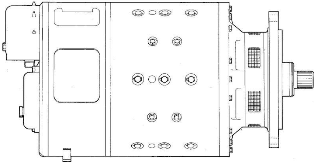
Fig. 1. Side elevation of 551A generator
