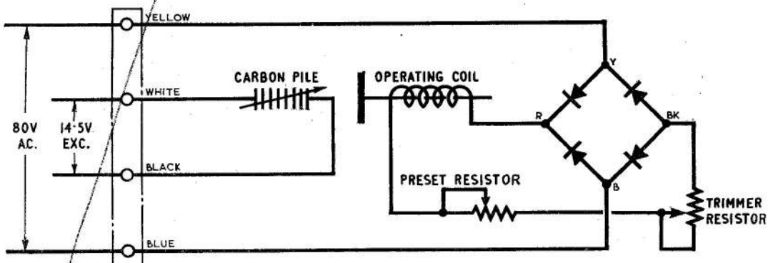
Fig. 1. Circuit diagram
