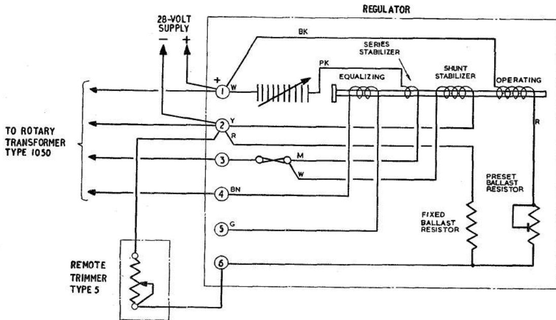
Fig. 2. Circuit diagram
