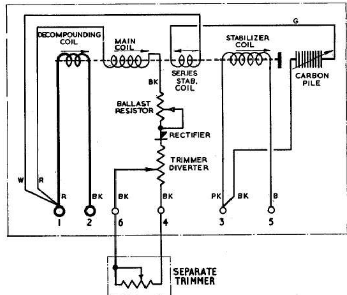
Fig. 3. Circuit diagram
