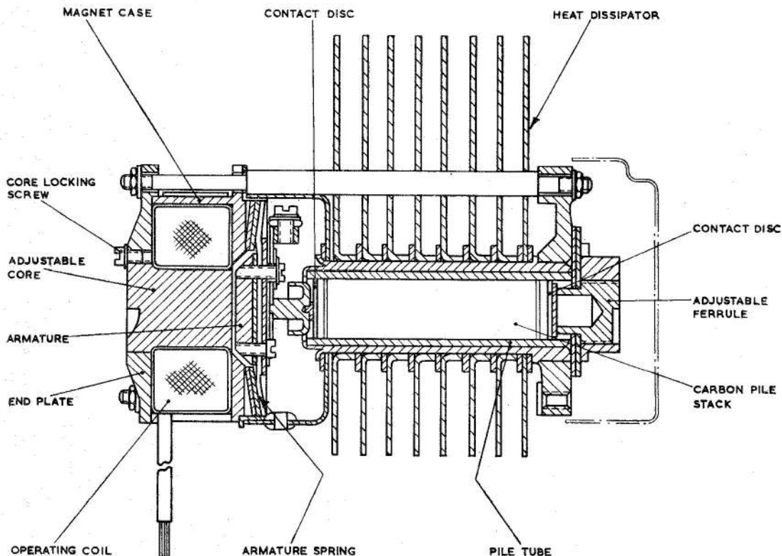
Fig. 2. Sectional view of regulator
