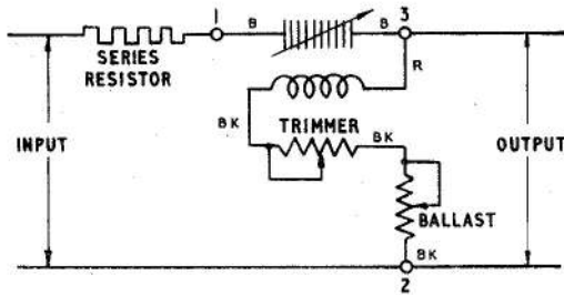
Fig. 3. Circuit diagram
