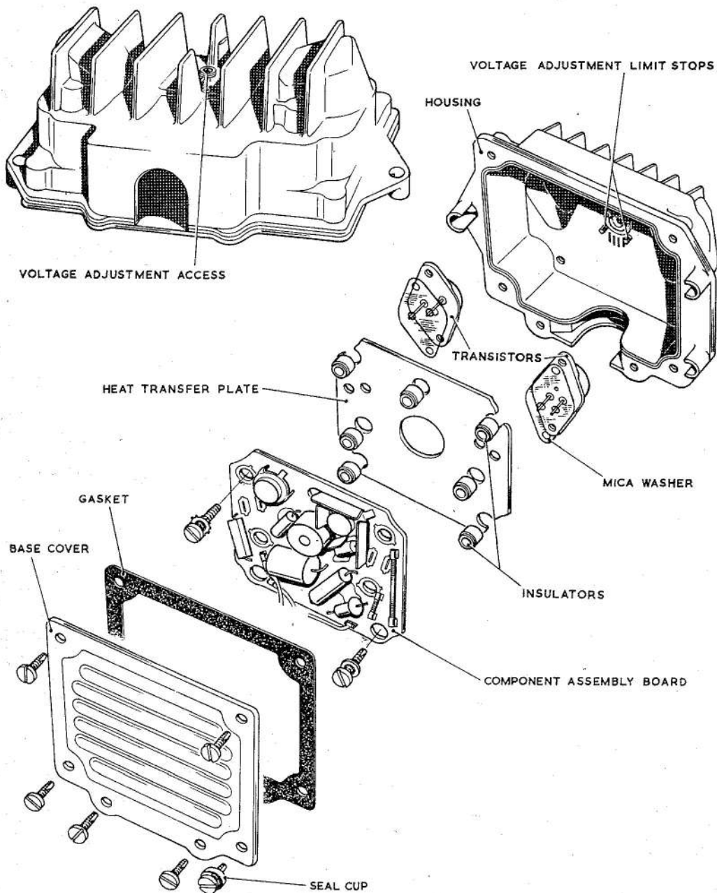
Fig. 2. Exploded view of regulator
