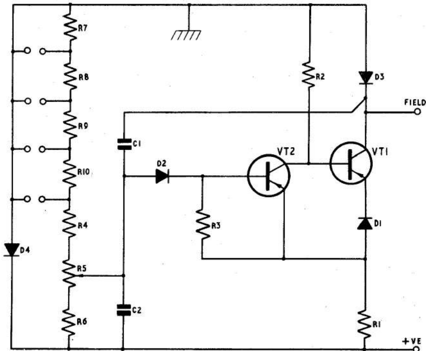
Fig. 3. Circuit diagram
