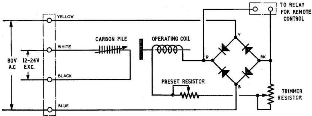
Fig. 1. Circuit diagram
