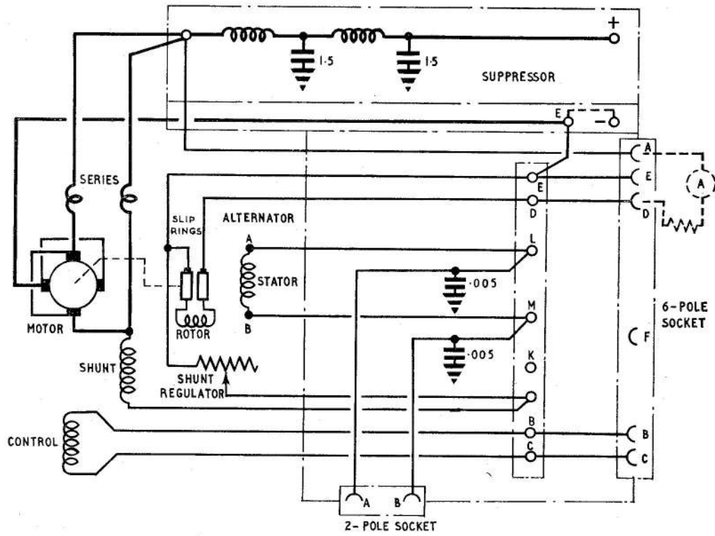
Fig. 2. Circuit diagram
