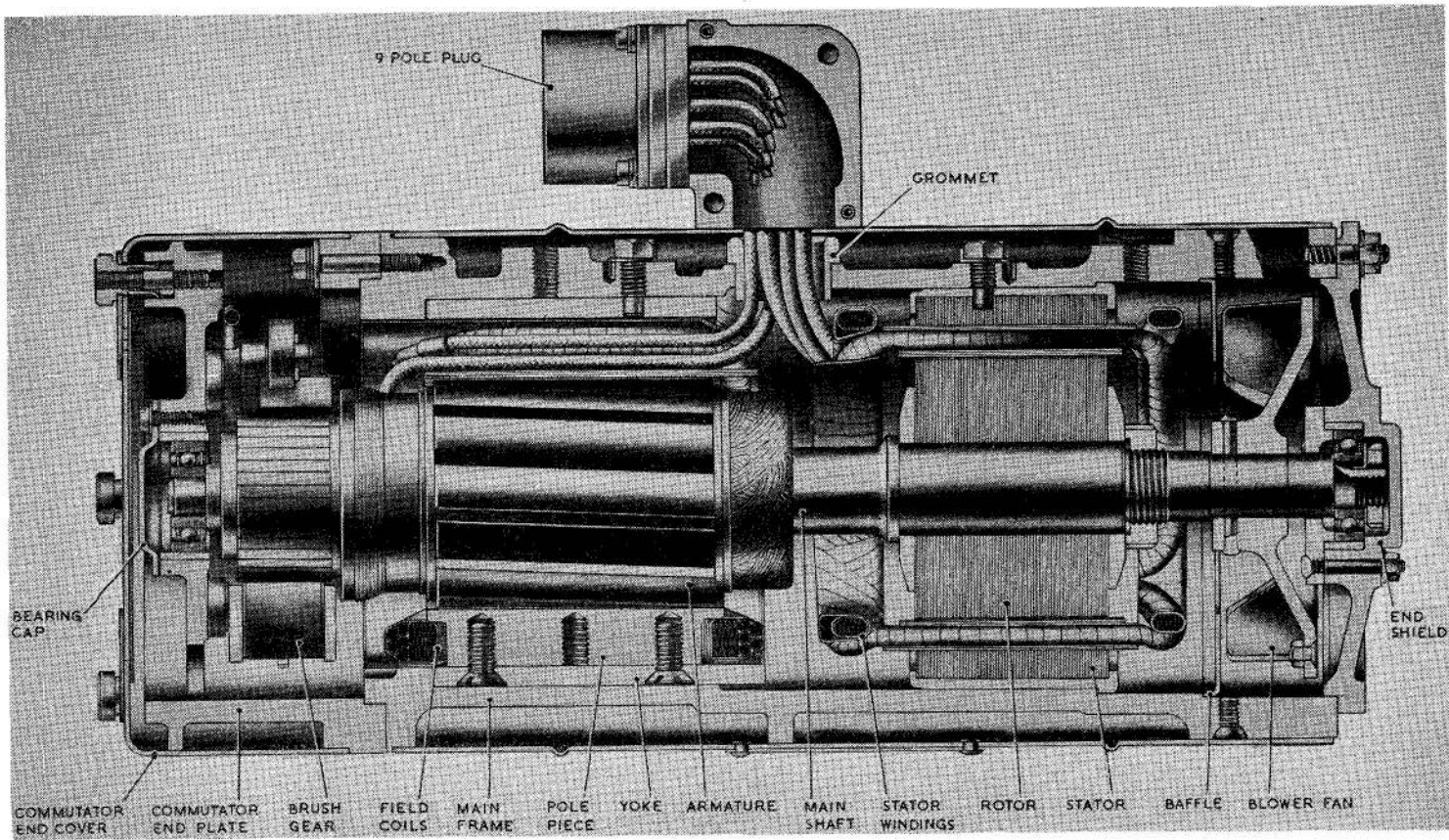
Fig. 2. Sectioned view
