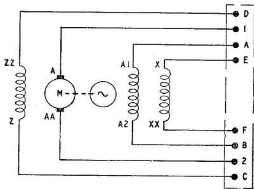
Fig. 3. Circuit diagram
