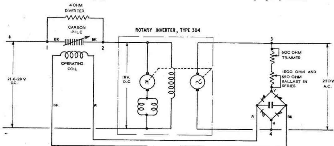
Fig. 3. Circuit diagram of rotary inverter, Type 304, with carbon pile regulator, Type 69
