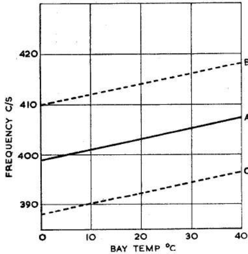
Fig. 2. Frequency/bay temperature characteristics
