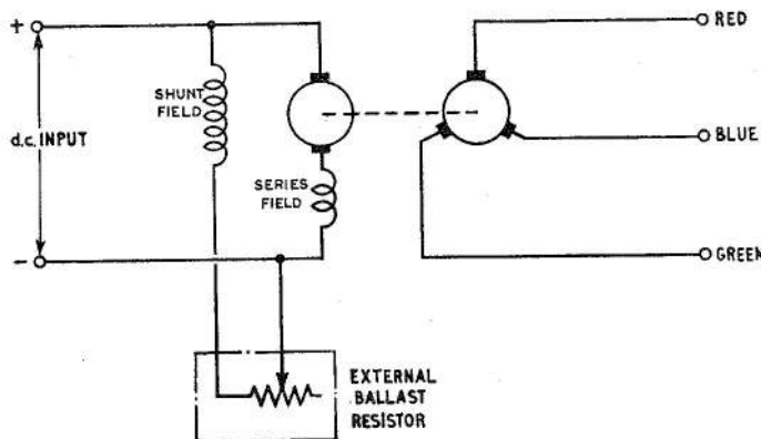
Fig. 1. Circuit diagram
