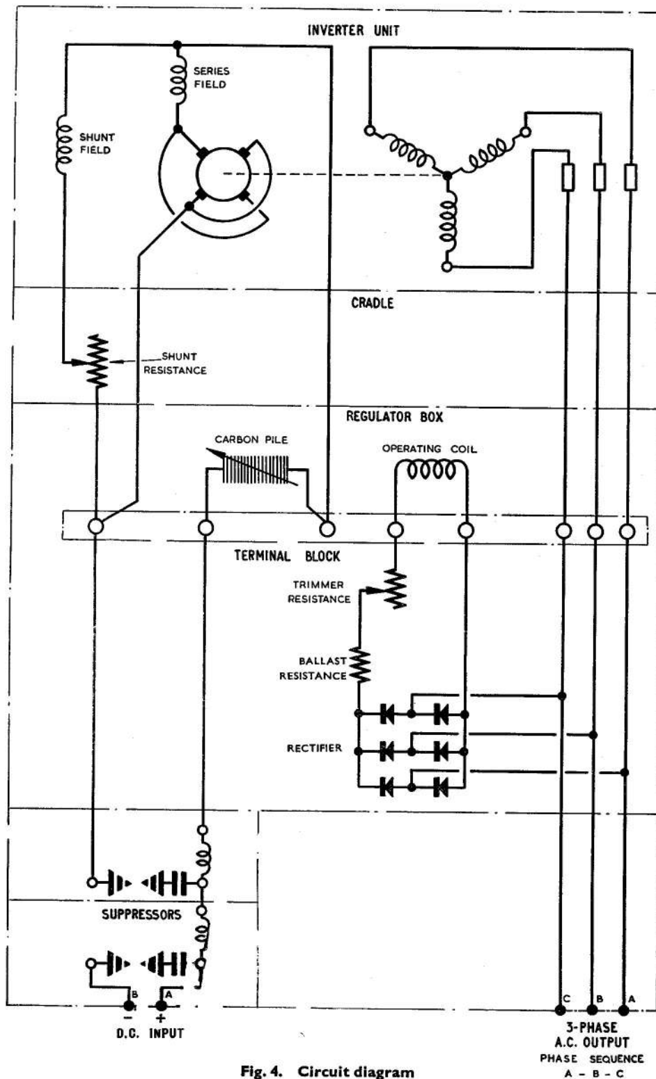
Fig. 4. Circuit diagram
