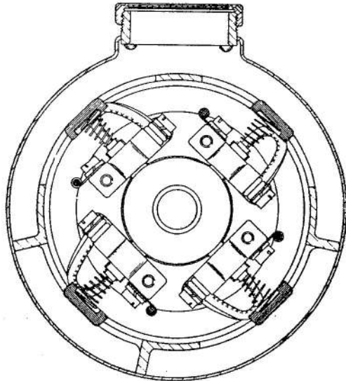
Fig. 3. Sectional view of brushgear (Type 201 shown)
