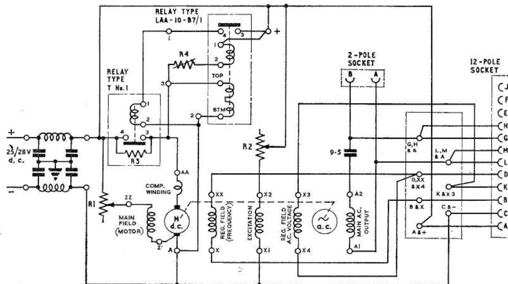
Fig. 1. Circuit diagram
