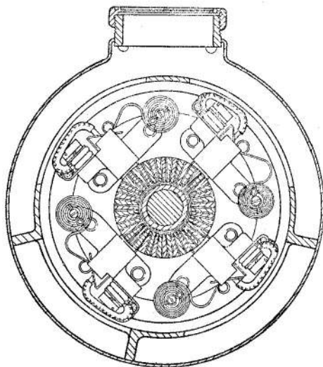
Fig. 2. Sectional view of brushgear
