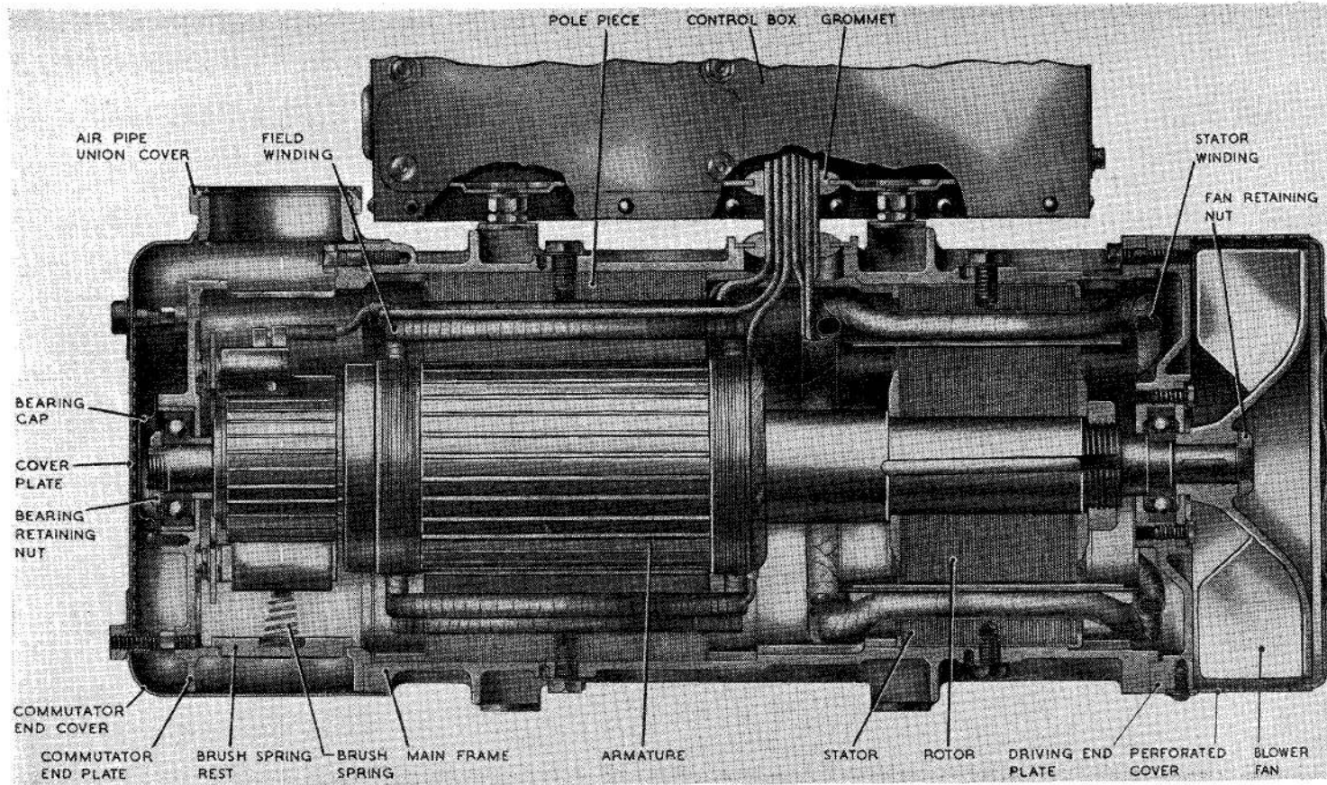
Fig. 2. Sectional view of inverter (Type 201 shown)
