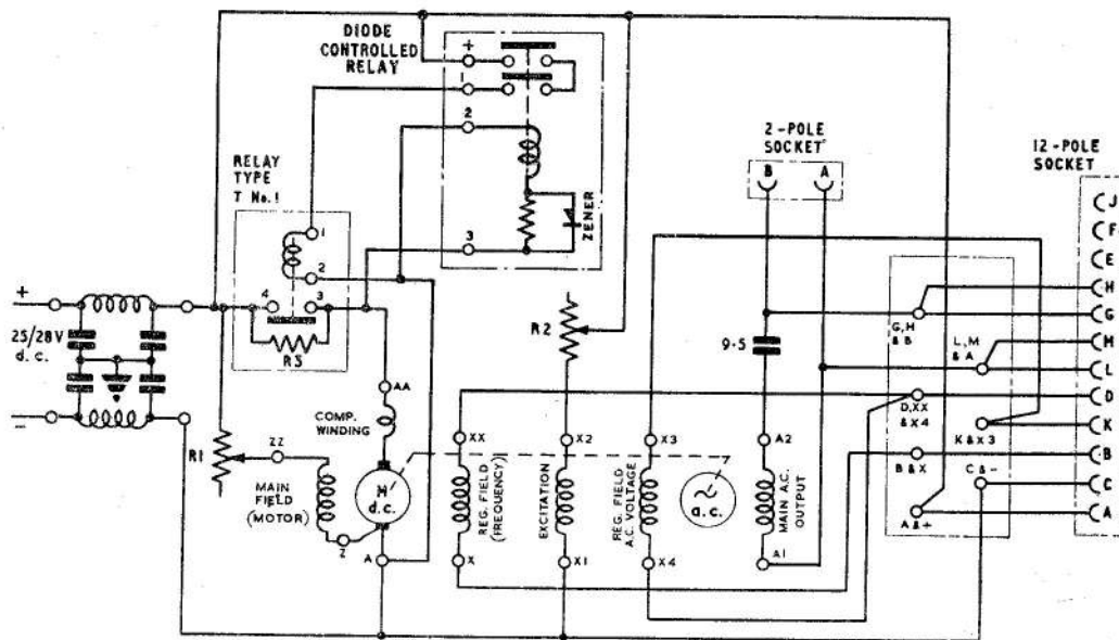
Fig. 1. Circuit diagram
