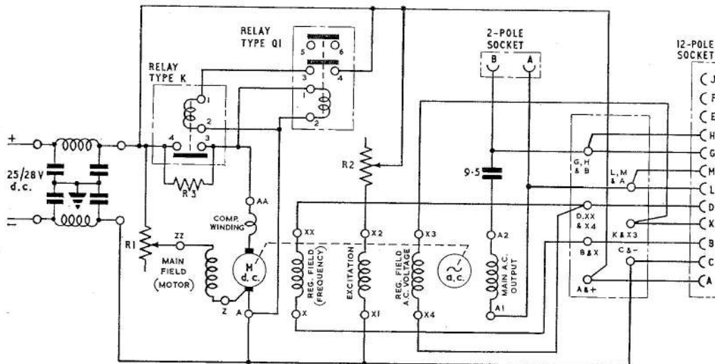
Fig. 4. Circuit diagram (Type 201 shown)
