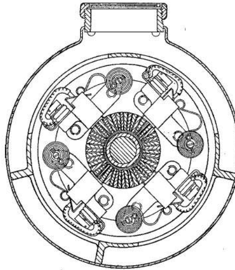
Fig. 1. Sectional view of brushgear
