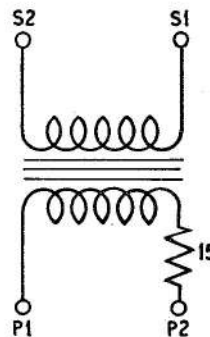
Fig. 3. Circuit diagram for Form B4/2
