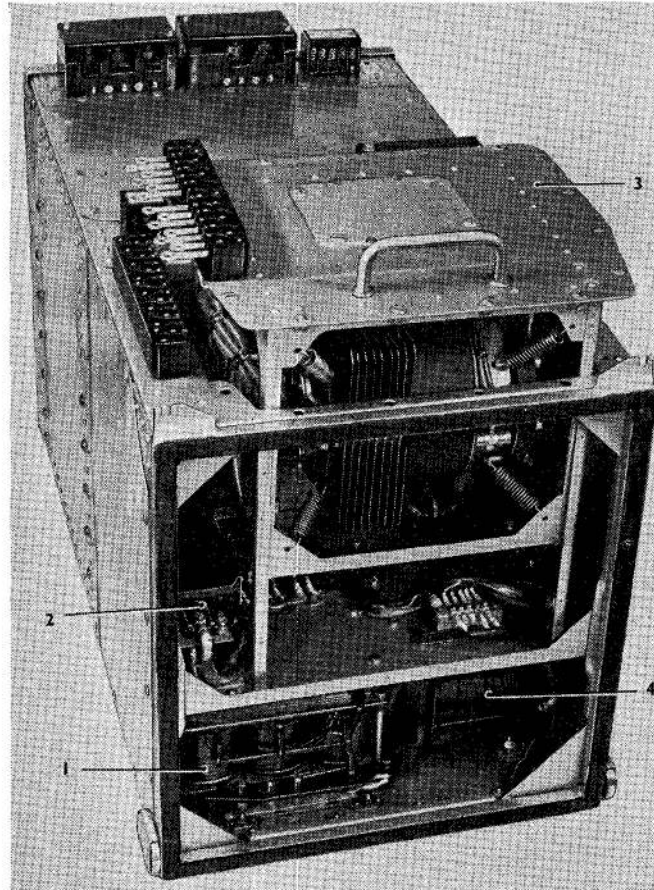
1 TRANSFORMER, TR.2 2 CONTACTORS, RL.3 AND RL.4 3 REGULATOR UNIT ASSEMBLY 4 TRANSDUCTOR, TD.1
