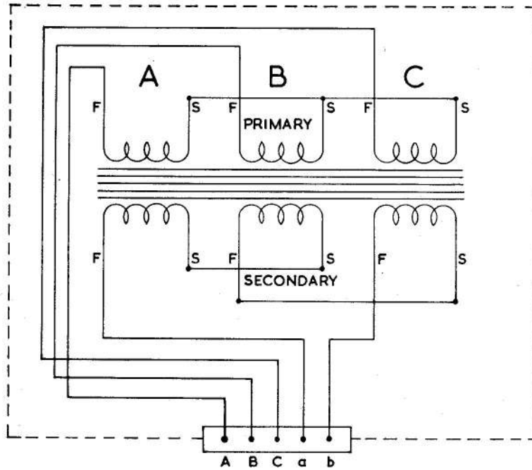
Fig. 2. Circuit diagram
