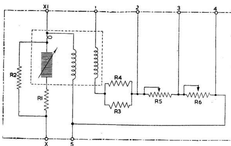
Fig. 5. Circuit diagram
