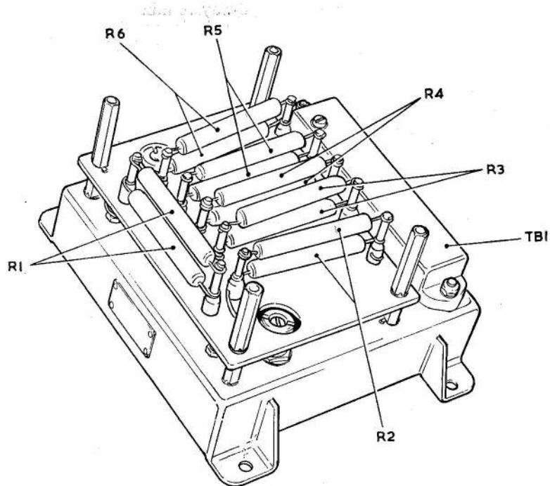
Fig. 2. Layout of components (top cover removed)
