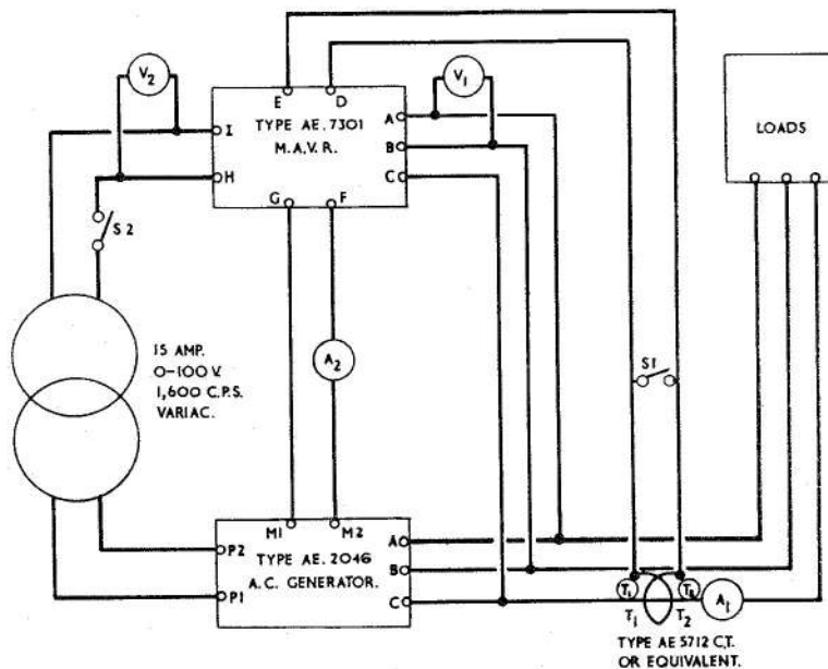
Fig. 6. Test circuit
