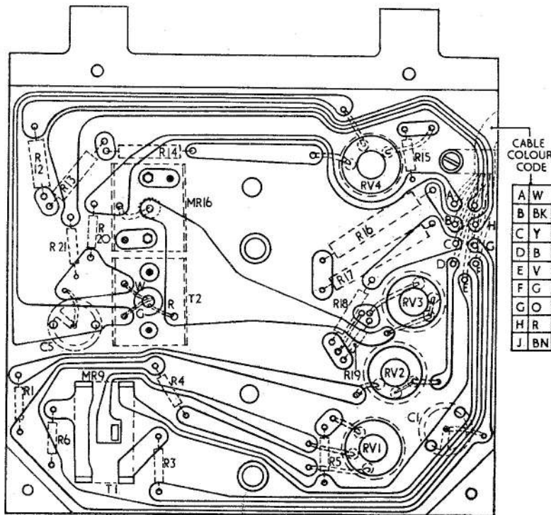
Fig. 4. Printed circuit
