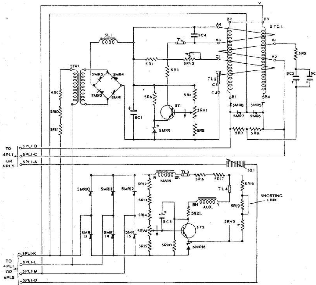
Fig. 5. Circuit diagram
