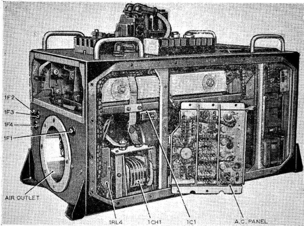
Fig. 6. View with a.c. panel in position
