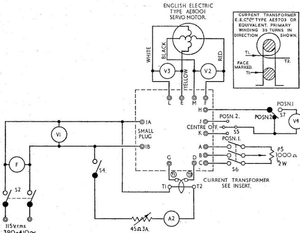
Fig. 5. Test circuit
