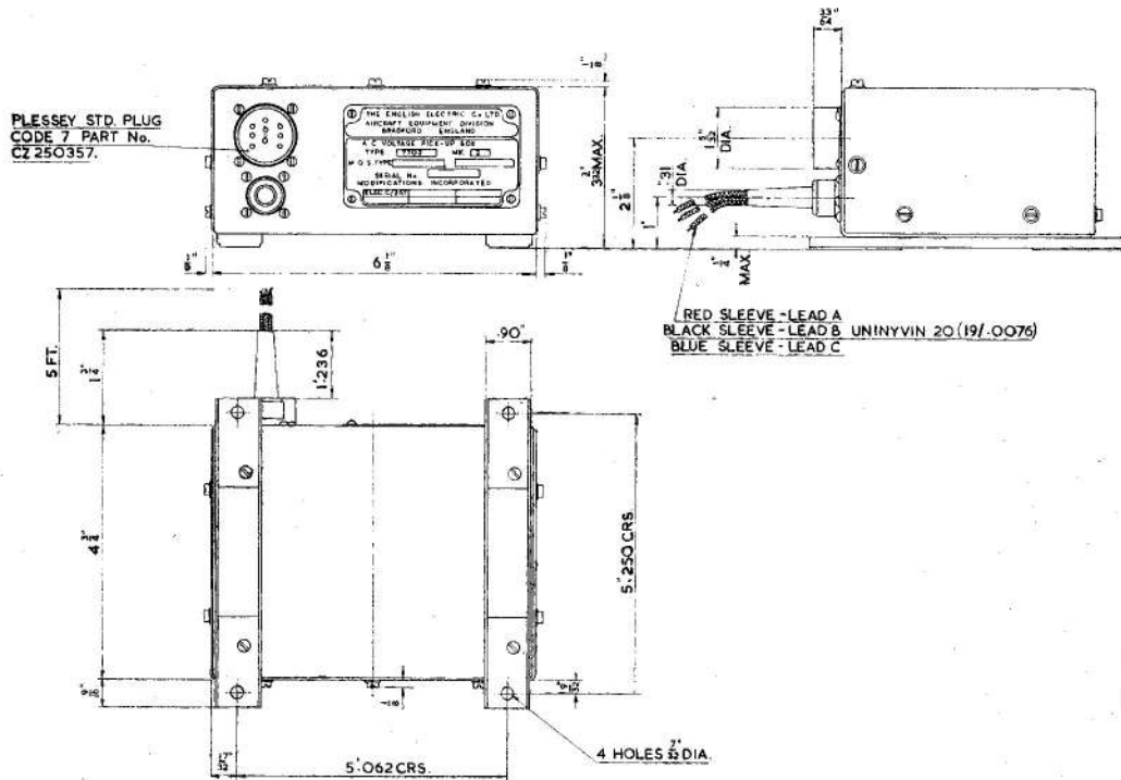
Fig. 4. Installation diagram
