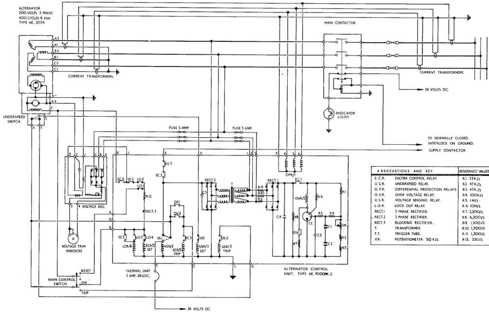
Fig 5 SCHEMATIC WIRING DIAGRAM RESTRICTED
