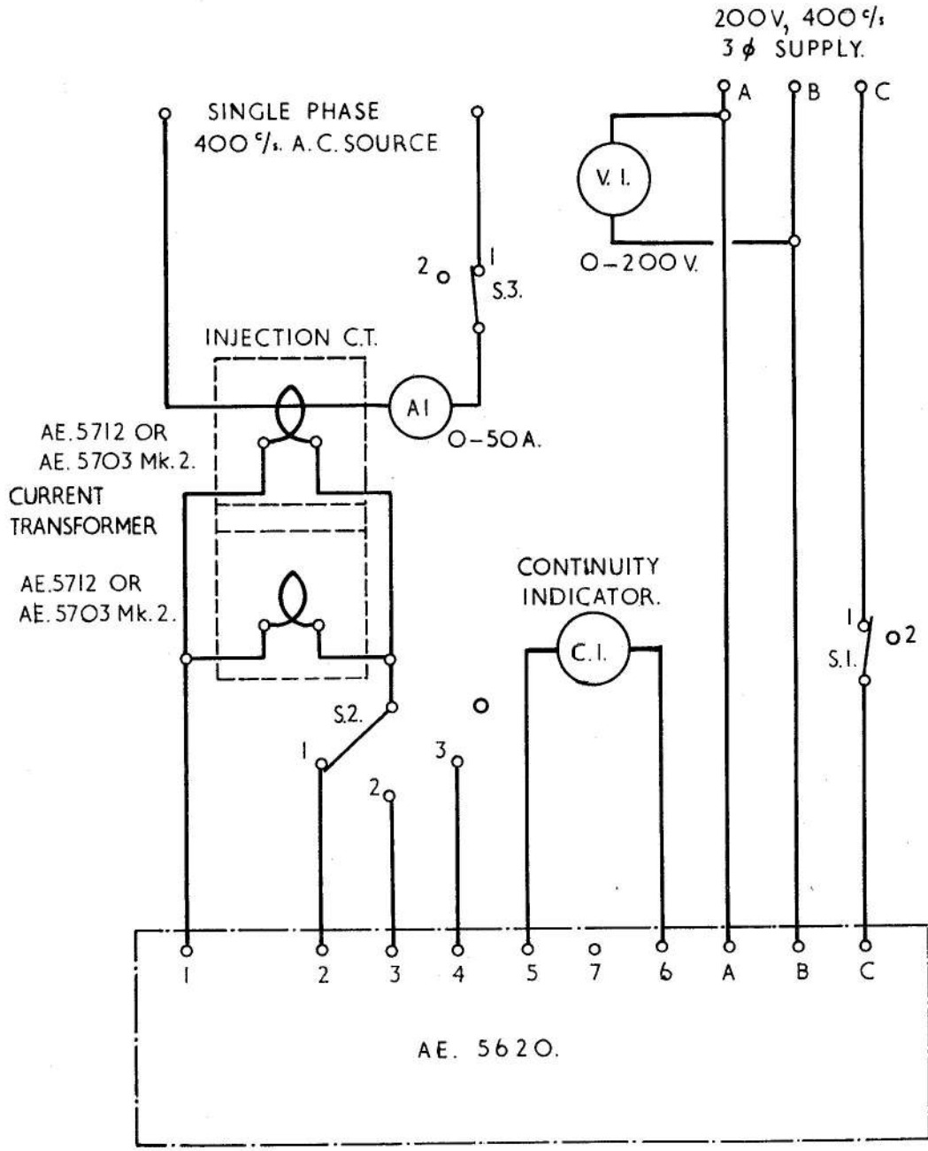
Fig. 4. Functional test circuit
