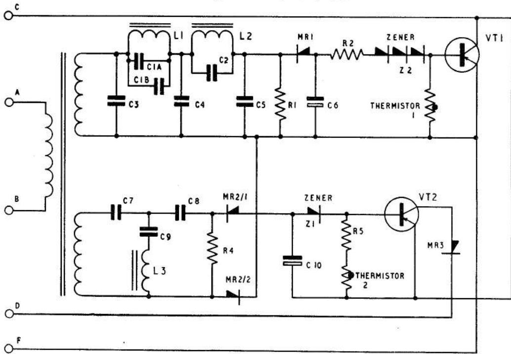
Fig. 4. Circuit diagram
