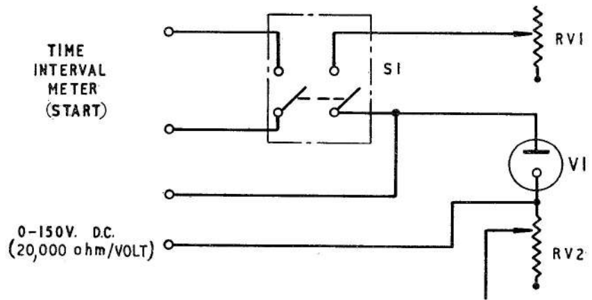
Fig. 7. Voltage control panel test circuit diagram
