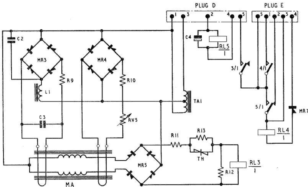
Fig. 6. Circuit diagram of under-frequency panel
