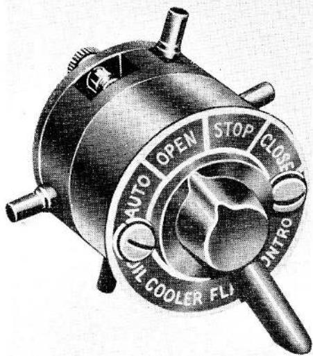
Fig. 1. Switch, A.E.I. type TD form 8
