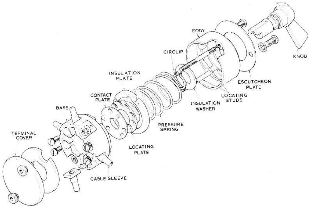
Fig. 3. Switch—exploded view
