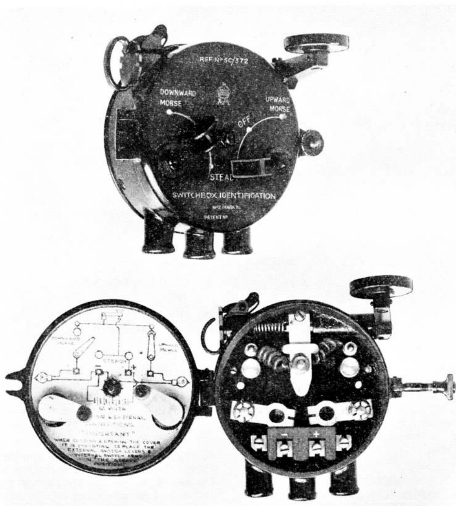
Fig. 1. Identification switchbox, Type B
