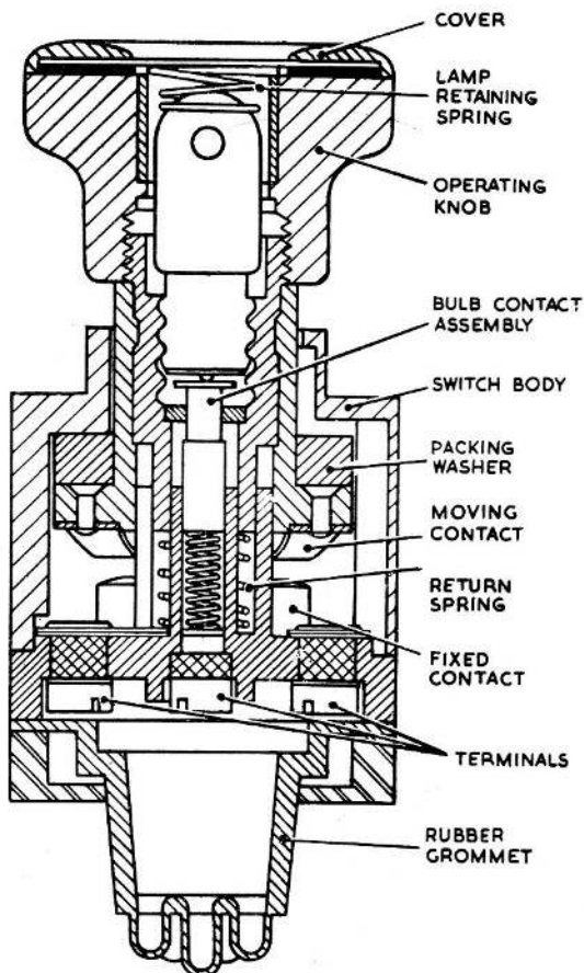
Fig. 2. Sectional view of switch
