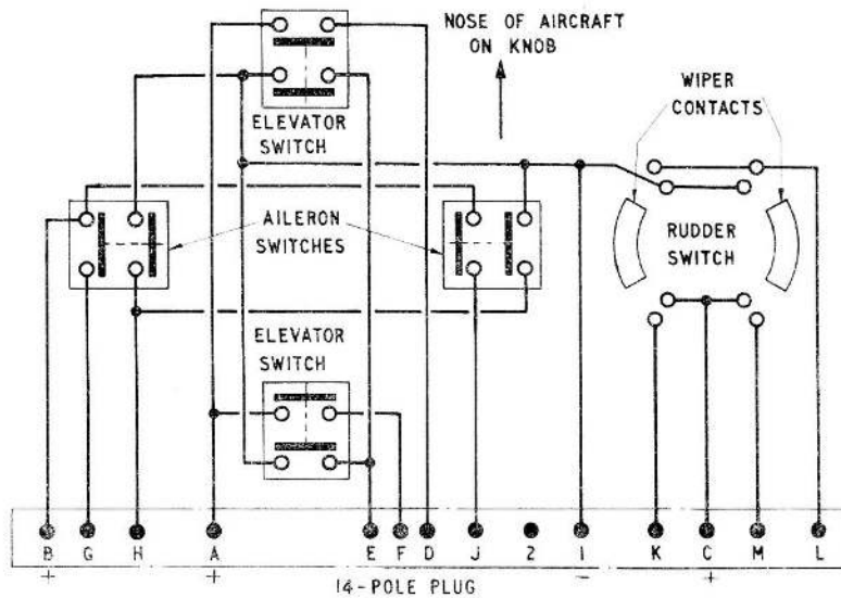
Fig. 3. Internal wiring diagram
