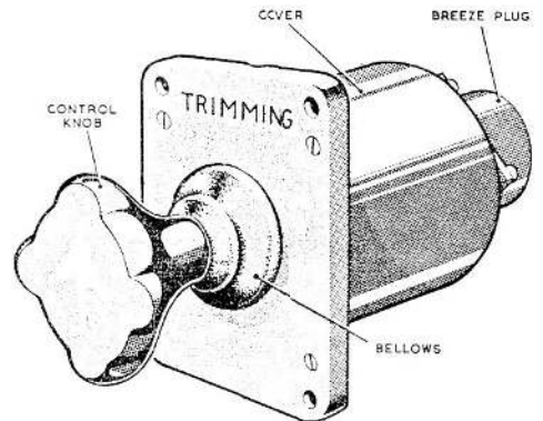
Fig. 1. Trim switch, Type TS231
