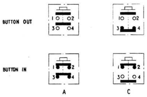
Fig. 4. Contact arrangement
