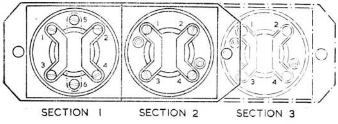
Fig. 3. Terminal arrangement
