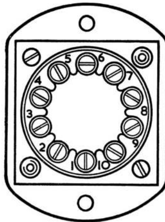
Fig. 3. Terminal arrangement
