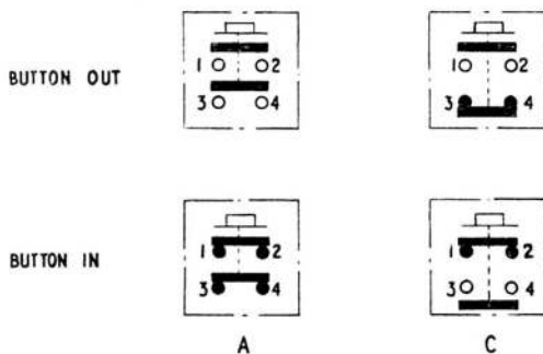
Fig. 4. Contact arrangement
