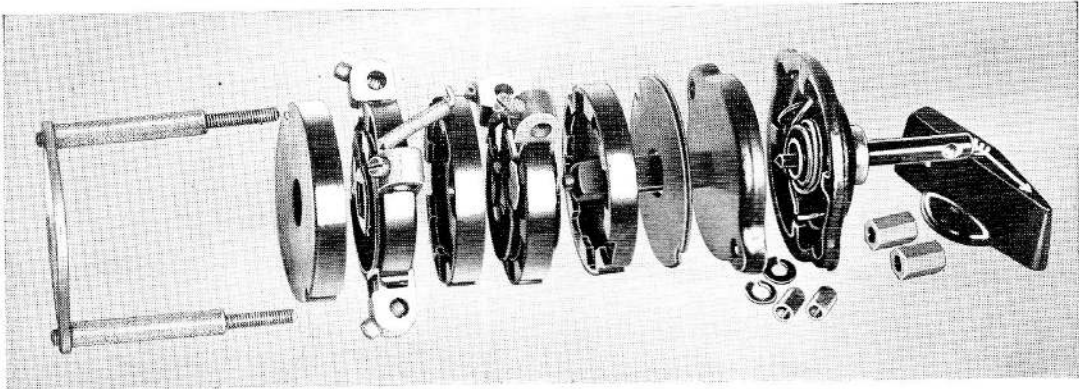
Fig. 3. Exploded view of switch
