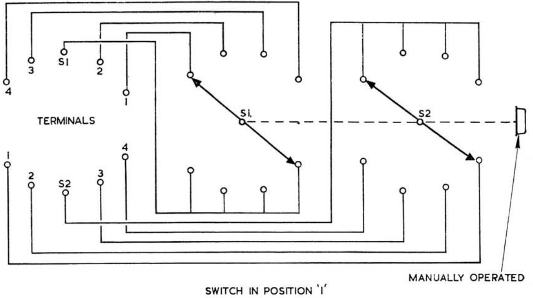
Fig. 3. Diagram of internal connections
