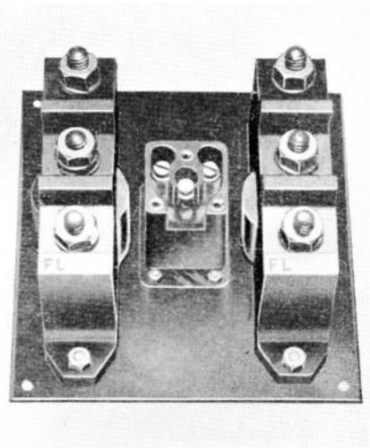
Fig. 2. Rear view of ground/flight switch
