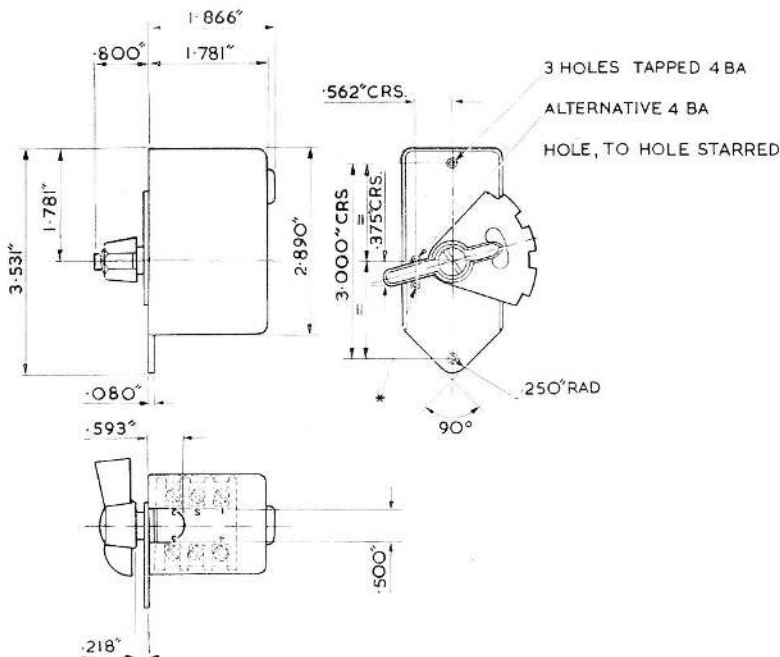
Fig. 3. Installation diagram
