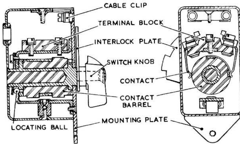
Fig. 2. Switch details
