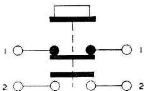
Fig. 2. Diagram of internal connections
