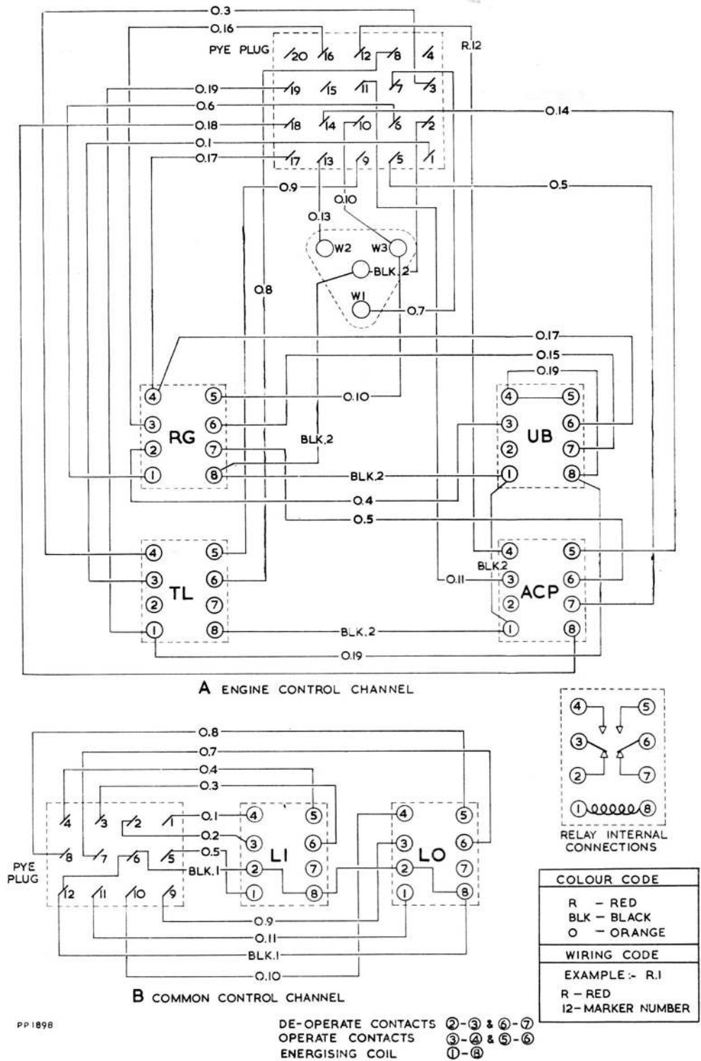
Fig. 8. Wiring diagram, engine and common control channels
