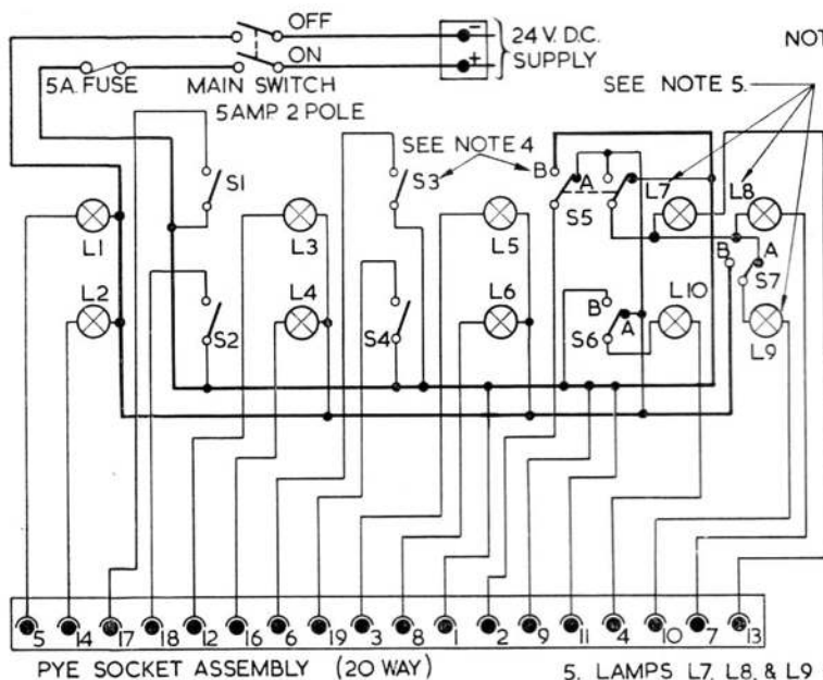
B TEST RIG FOR ENGINE CONTROL CHANNEL
