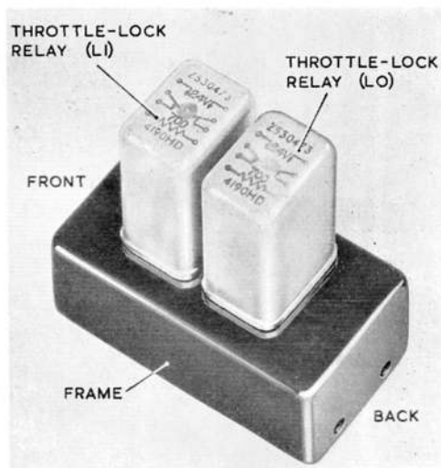
Fig. 4. Common control channel (cover removed)
