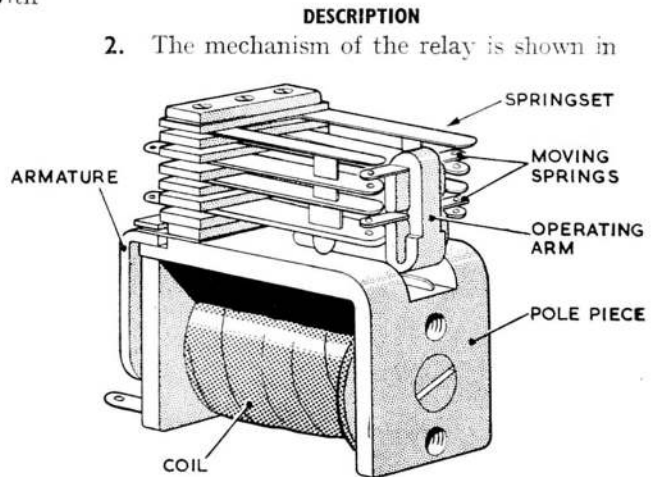
Fig. 2. Relay removed from its casing
