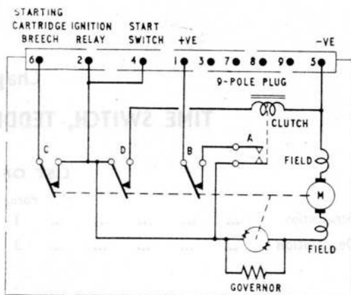
Fig. 2. Circuit diagram
