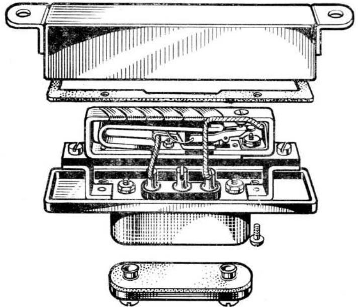
Fig. 1. Exploded view of thermostat unit
