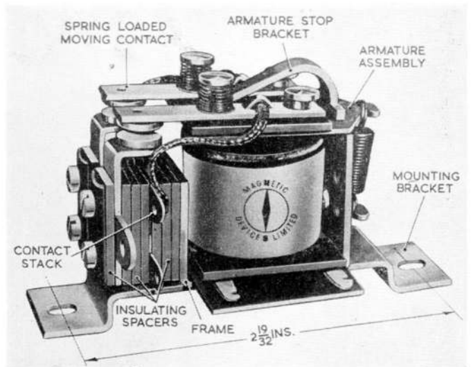
Fig. 1. Typical (155 Series) relay
