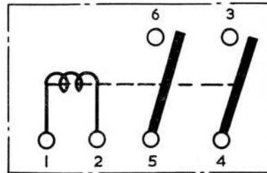
Fig. 4. Circuit diagram
